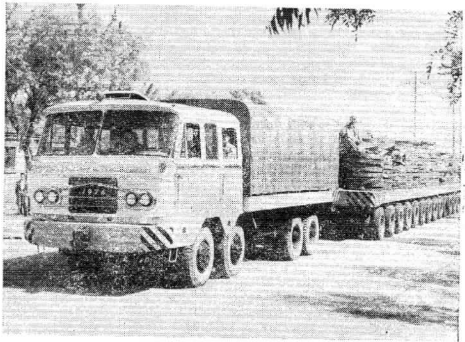
The 400-ton platform trailer produced by workers of Tsangchow.
